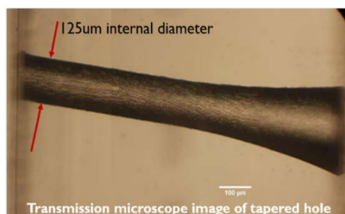
Figure 2: Hole with 8-degree tapered entrance for smooth fiber insertion.
